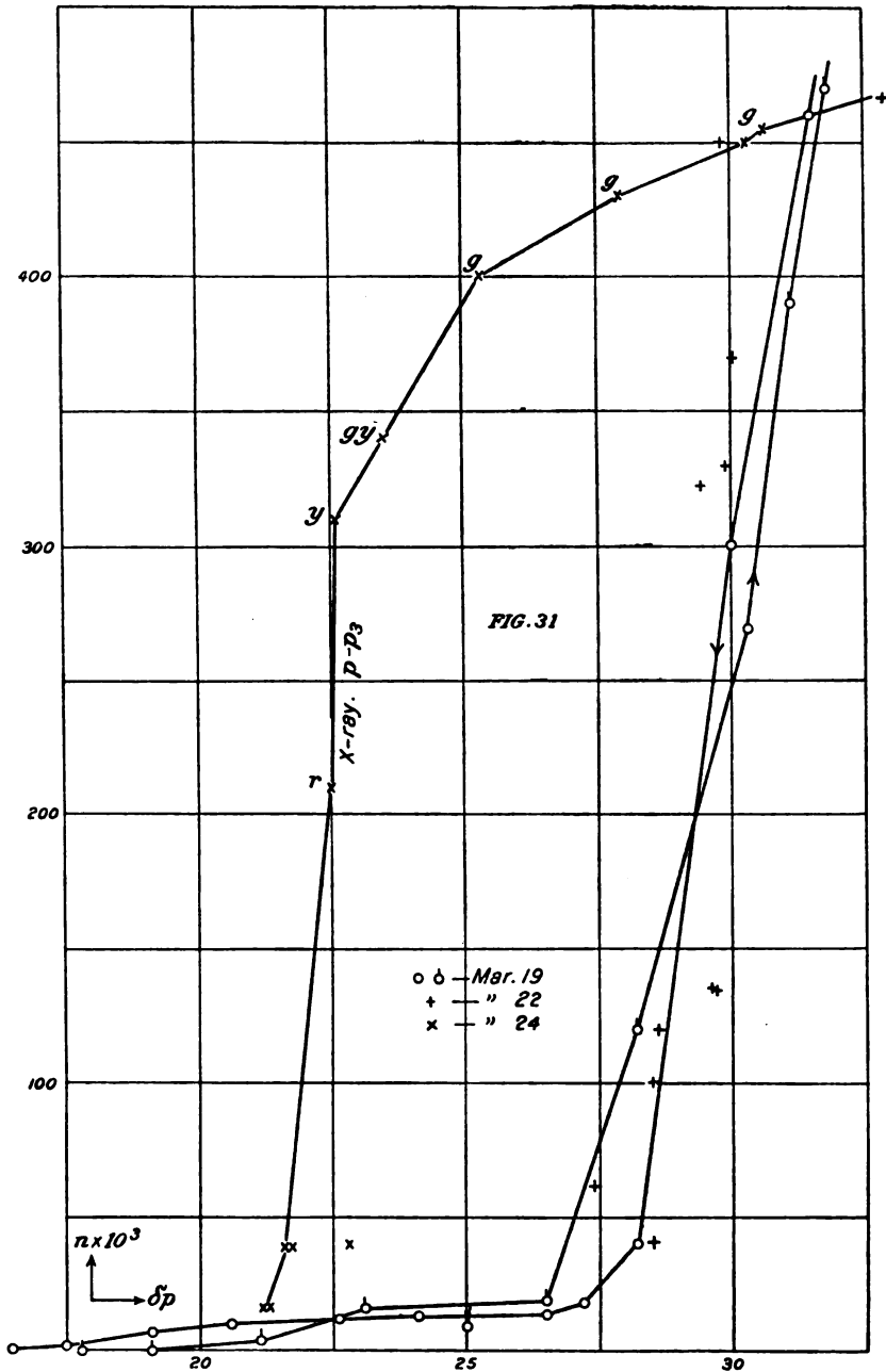
FIG. 31.—Nucleations (*) observed in dust-free air and dust-free X-air at different exhaustions ( \delta p ); 4-inch pipes. Table 21.
